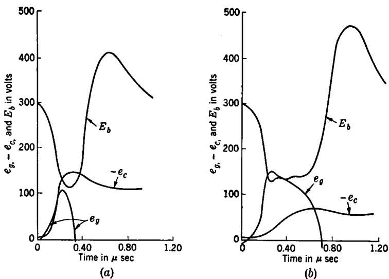
Fig. 14-25.—Typical pulse shapes obtained from a regenerative pulse generator employing a 6SN7 triode, a 132AW2 pulse transformer (see Table 13-2) for which R = 25,000 ohms, and E_{bb} = 300 volts. (a) C = 235 \mu\text{mf} . (b) C = 2700 \mu\text{mf} .
